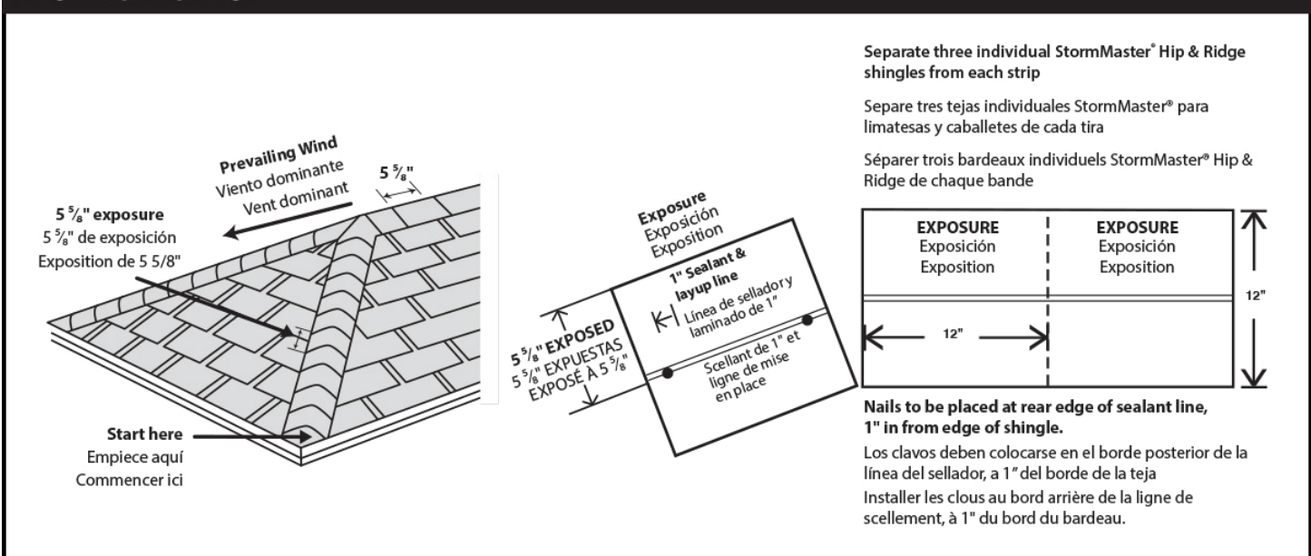
DIAGRAM 6 HIP & RIDGE
